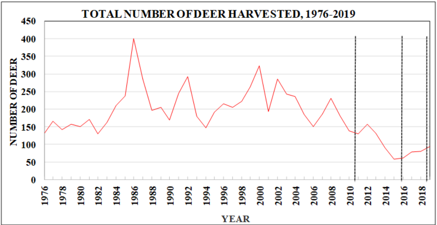
Figure 1. Line graph showing the total number of deer harvested at West Point from 1976 to 2019. Data included represents total deer from all seasons. Doe harvest was restricted by regulations, 2010-2016 including significantly restricted in 2015 and 2016. In 2019, a three-to-a-side antler point restriction was implemented.
