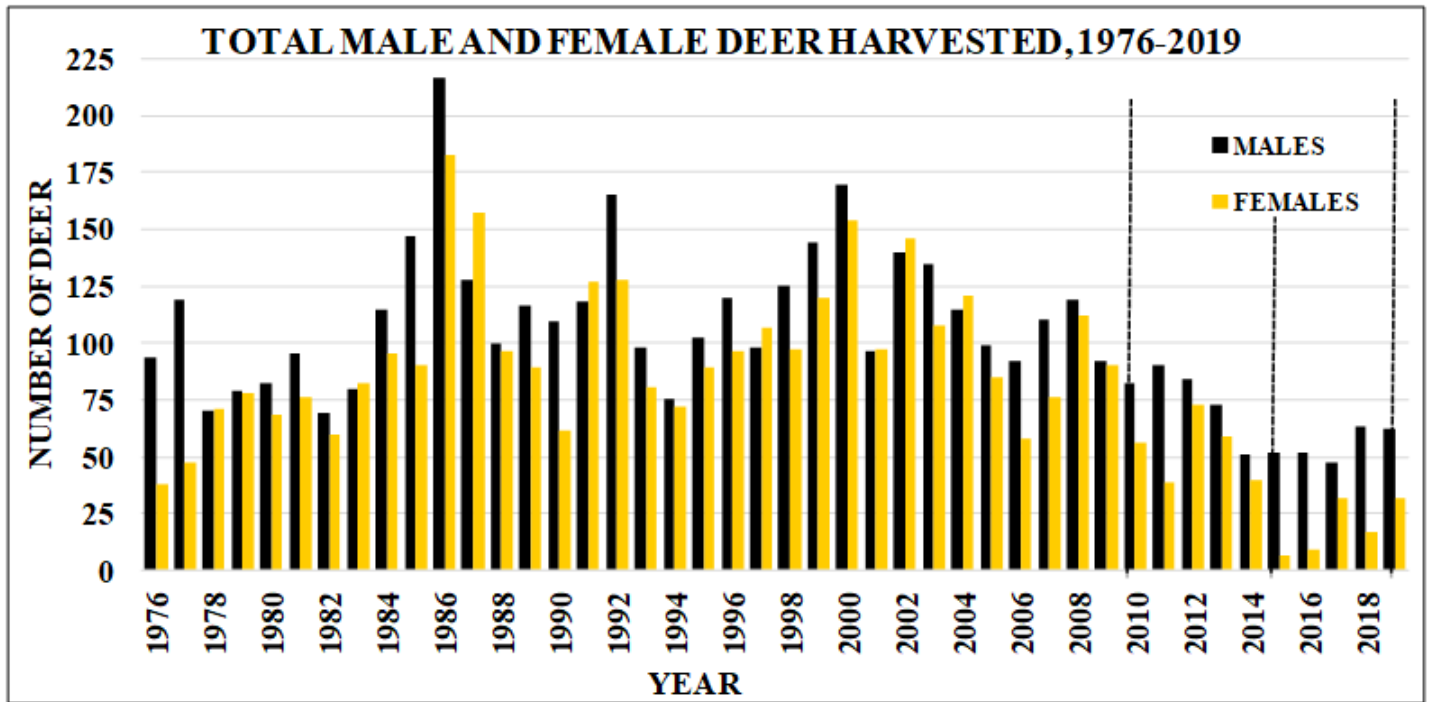
Figure 2. Bar Graph showing total numbers of male and female deer harvested at West Point from 1976 to 2019. Data included is from all seasons. Doe harvest was restricted by regulations, 2010-2016 including significantly restricted in 2015 and 2016. In 2019, a three-to-a-side antler point restriction was implemented.
